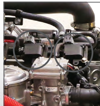
Coil over plug ignition design
