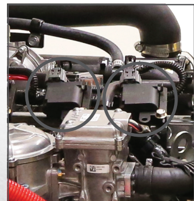
Coil over plug ignition design
